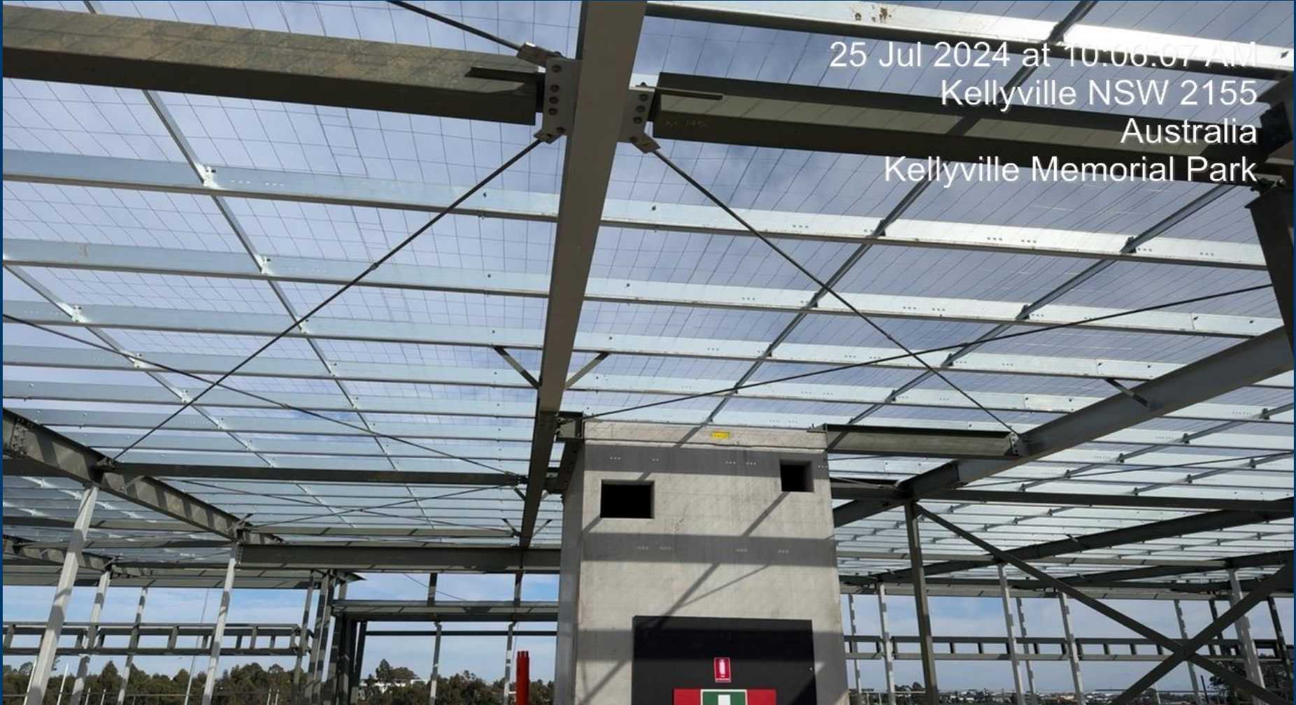
Building B – Installation of Roof Safety Mesh
