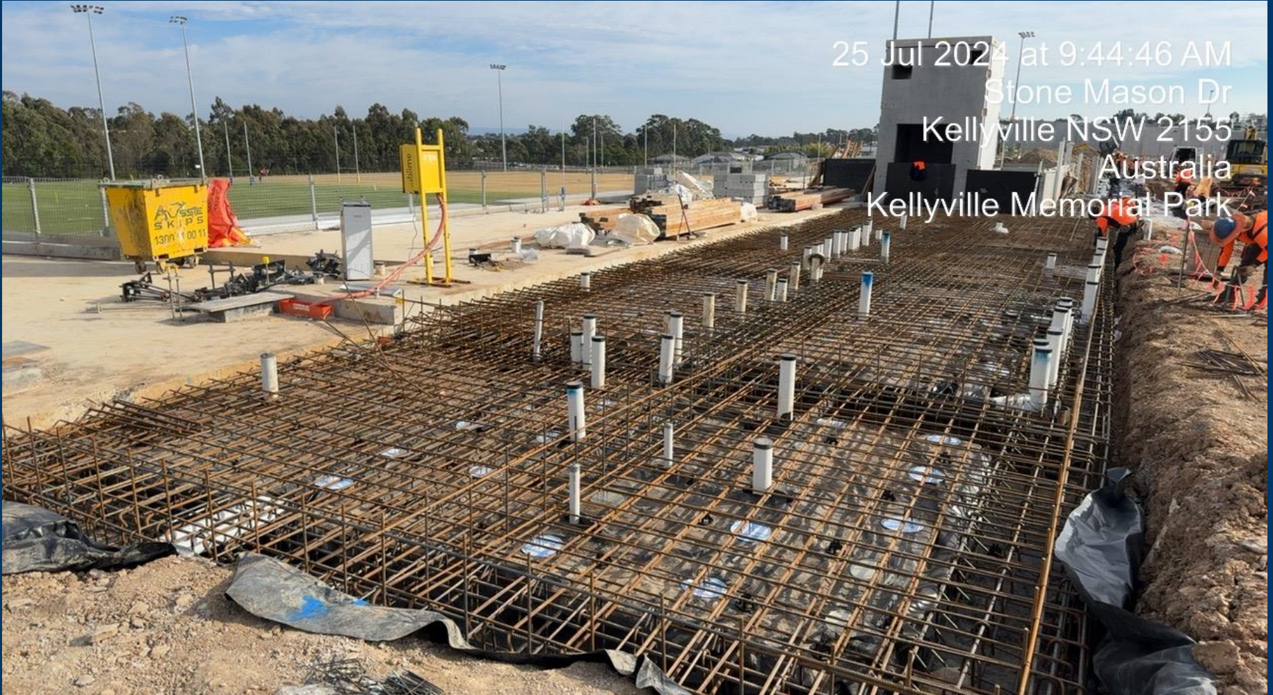
Building A – Upper Floor Pour 3 Steel fixing
